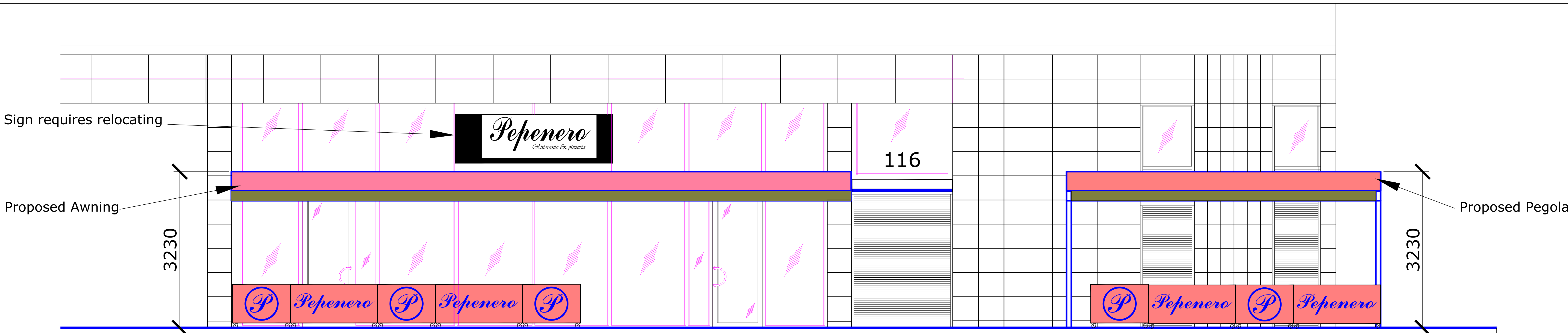
Proposed Elevation Scale 1:50
